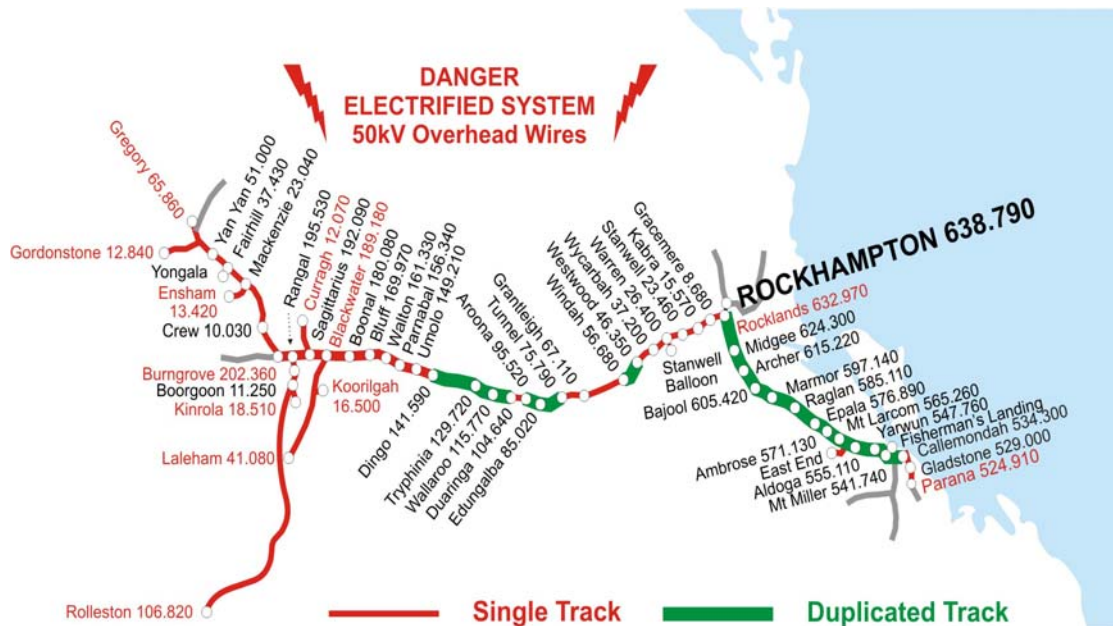
Figure 1.1 Nominated Network - BLACKWATER SYSTEM
