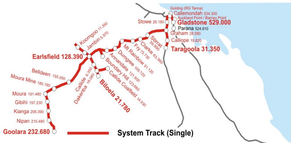
Figure 1.4 Nominated Network - MOURA SYSTEM
