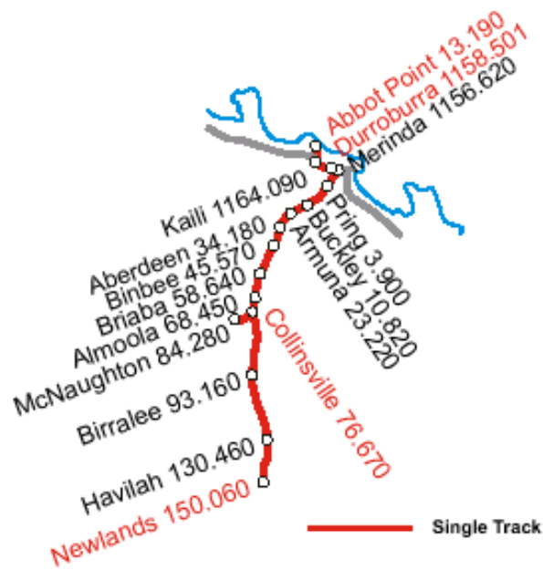
Figure 1.3 Nominated Network - NEWLANDS SYSTEM
